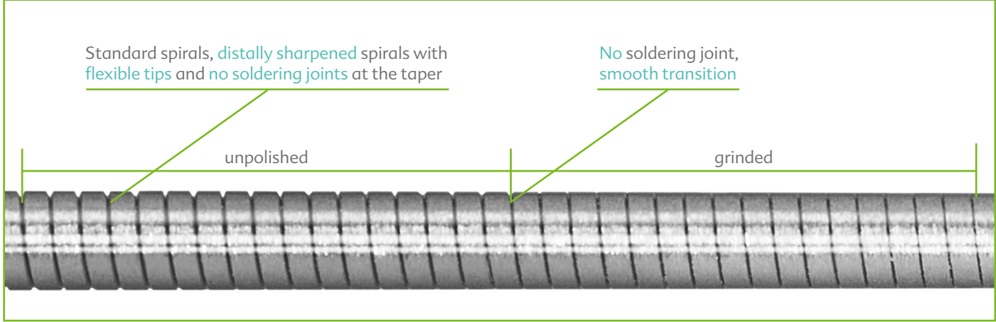
Distally sharpened spring (V)
